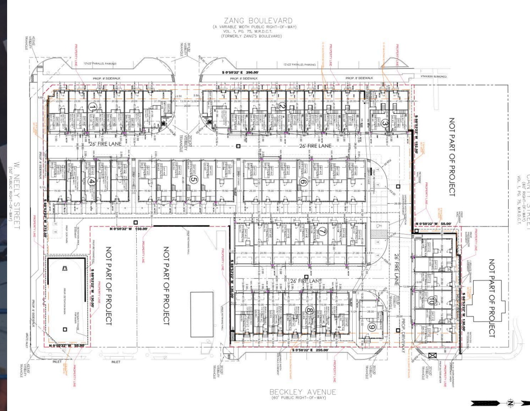
SITE PLAN
