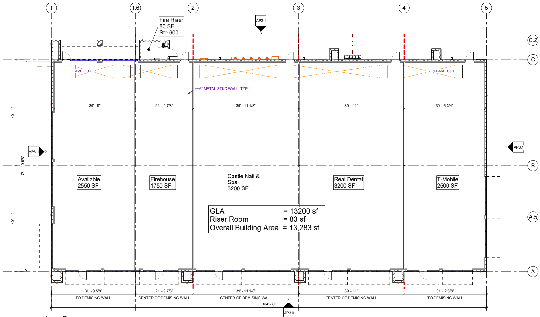
1 Lease Plan 1/8" = 1'-0"
