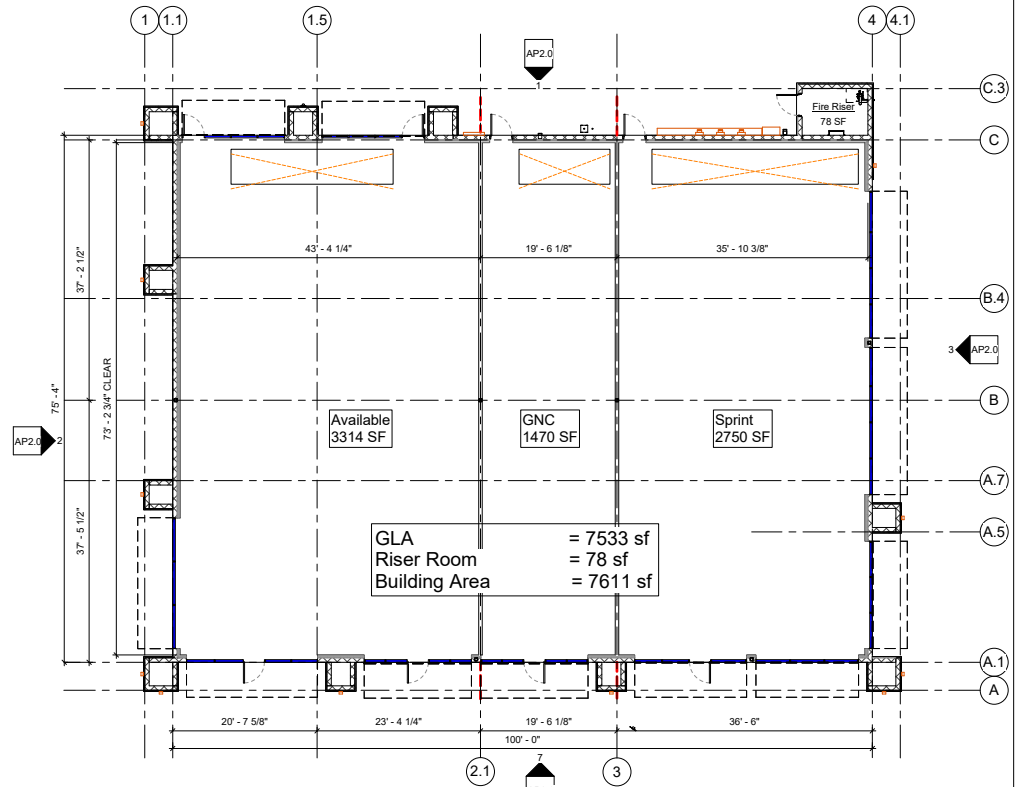
4 Lease Plan - Bldg 11A 1/8" = 1'-0"
