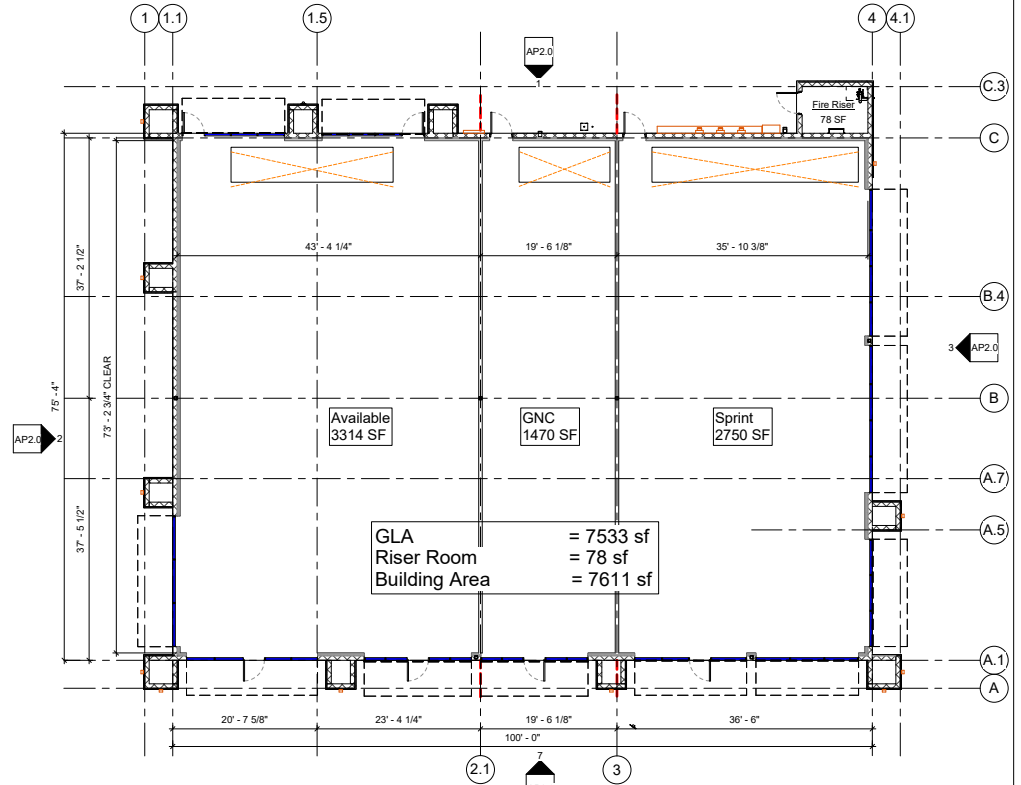
④ Lease Plan - Bldg 11A 1/8" = 1'-0"
