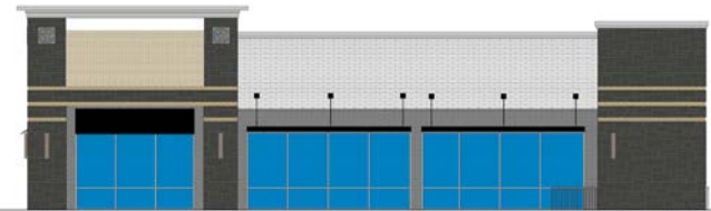
③ East Elevation 1/8" = 1'-0"
