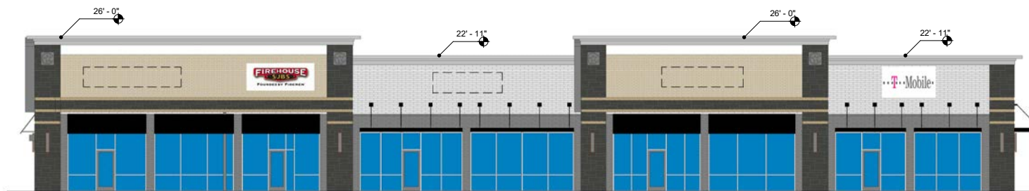
4 South Elevation 1/8" = 1'-0"
