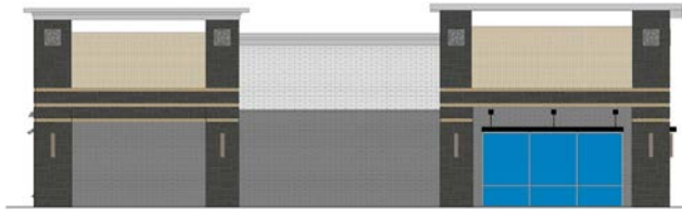
② West Elevation 1/8" = 1'-0"
