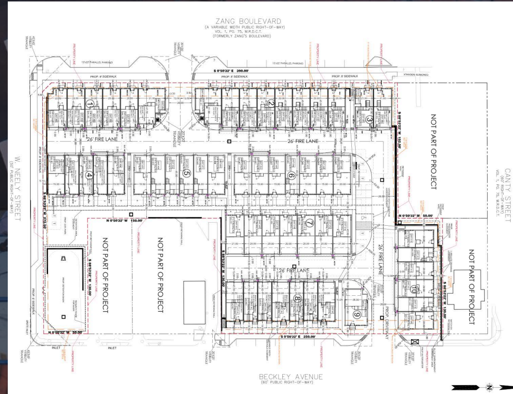
SITE PLAN
